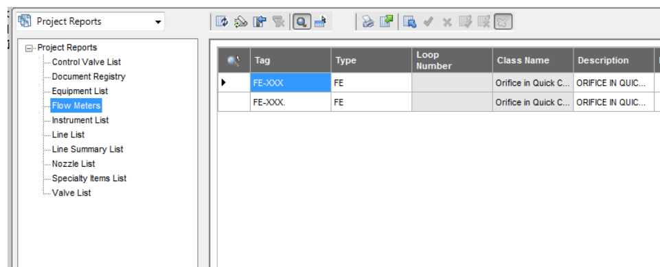
Figure 253: View Report
