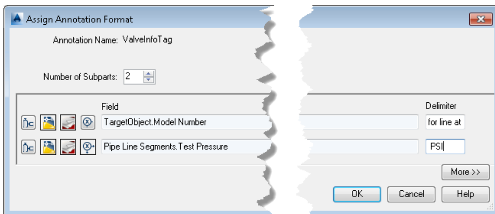
Figure 136: Annotation with Related Property
