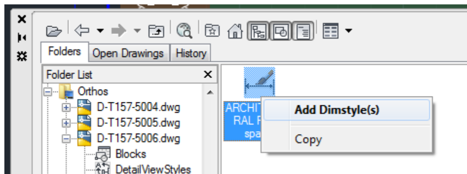
Figure 228: Add Dimstyle
