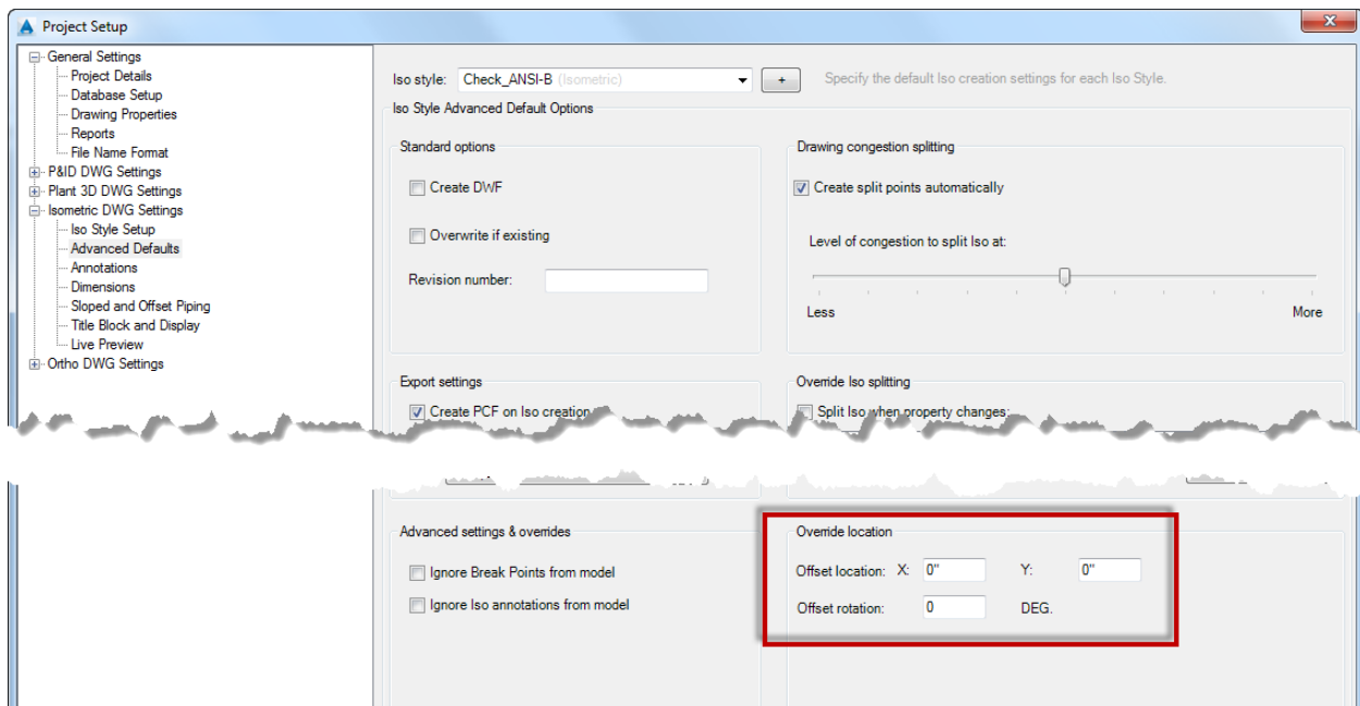
Figure 167: Coordinate Overrides
